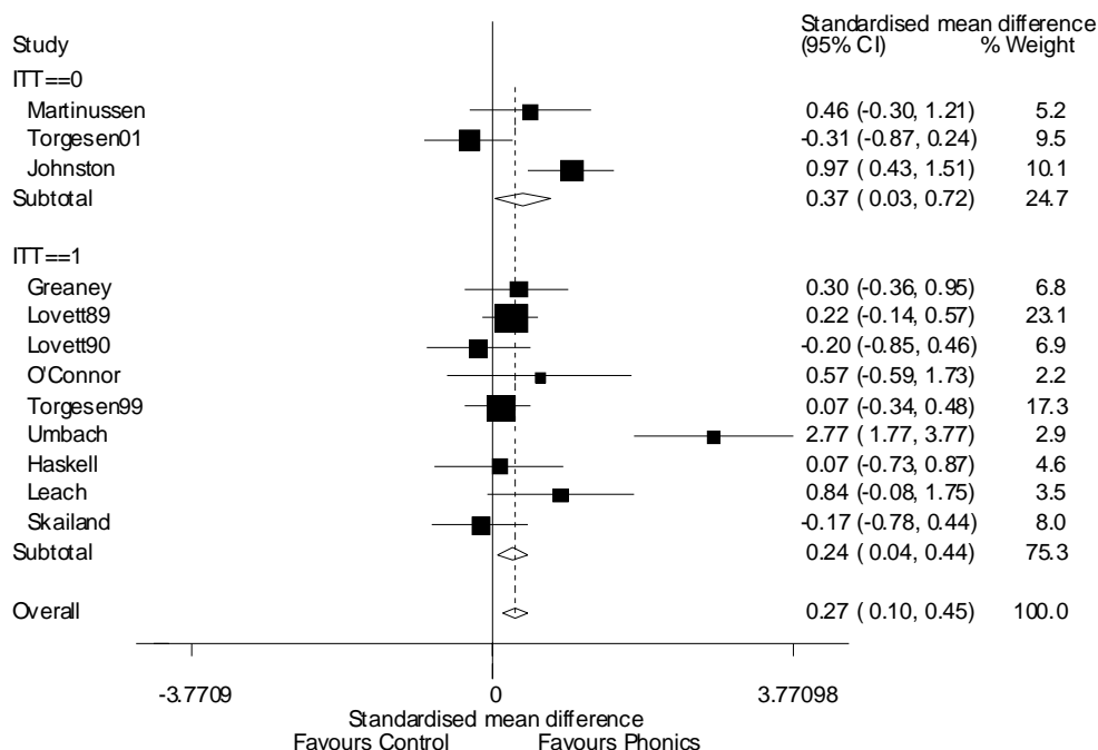
Figure 3: Main meta-analysis subdivided by ITT or no-ITT
