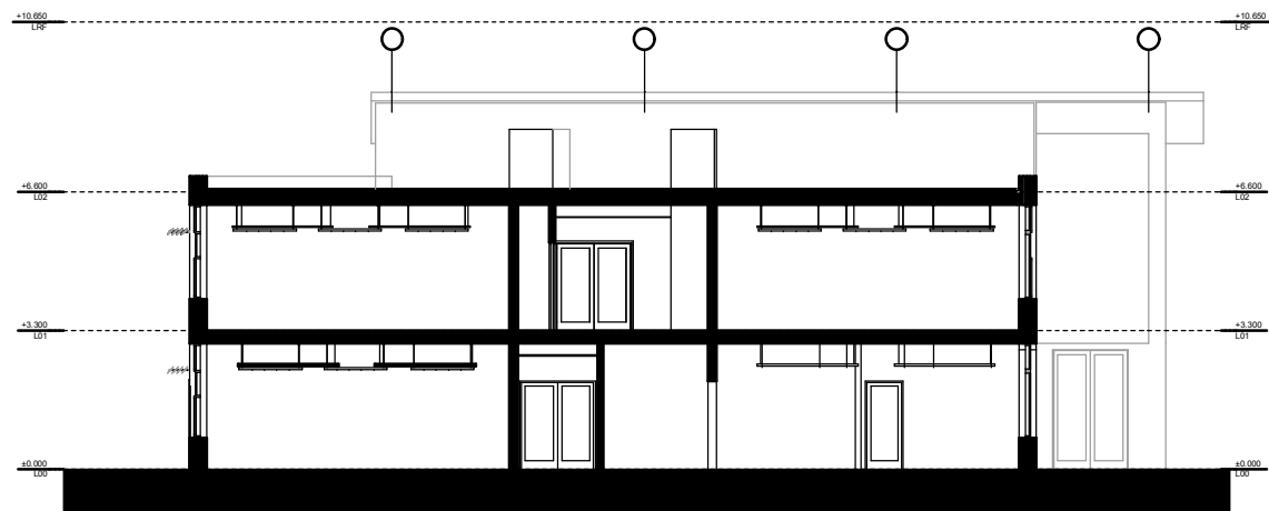
SECTION BB
