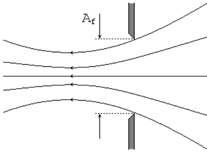
Figure D-3: Streamlines through a 'sharp-edged' orifice
