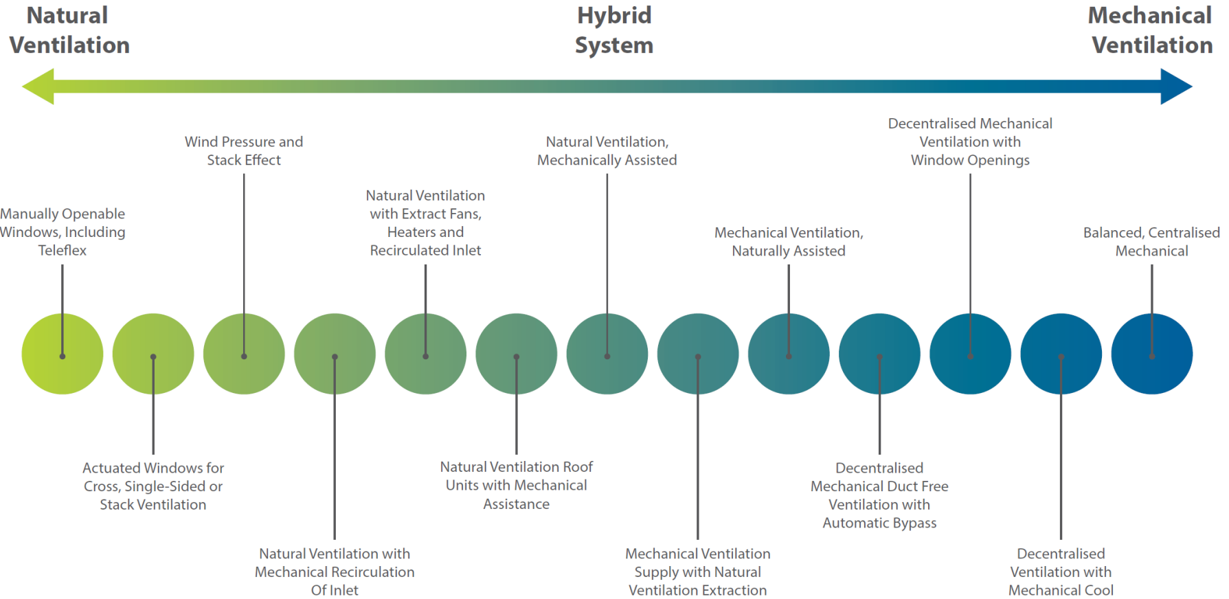
Figure 1-2 Types of ventilation system
