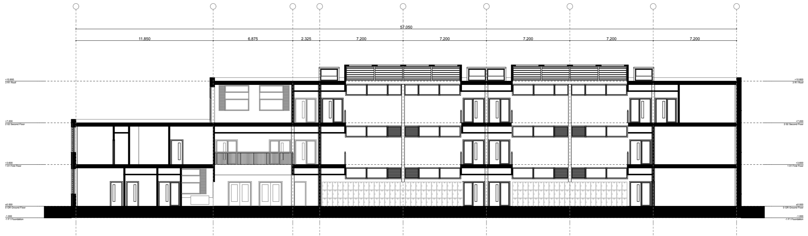
Section CC
