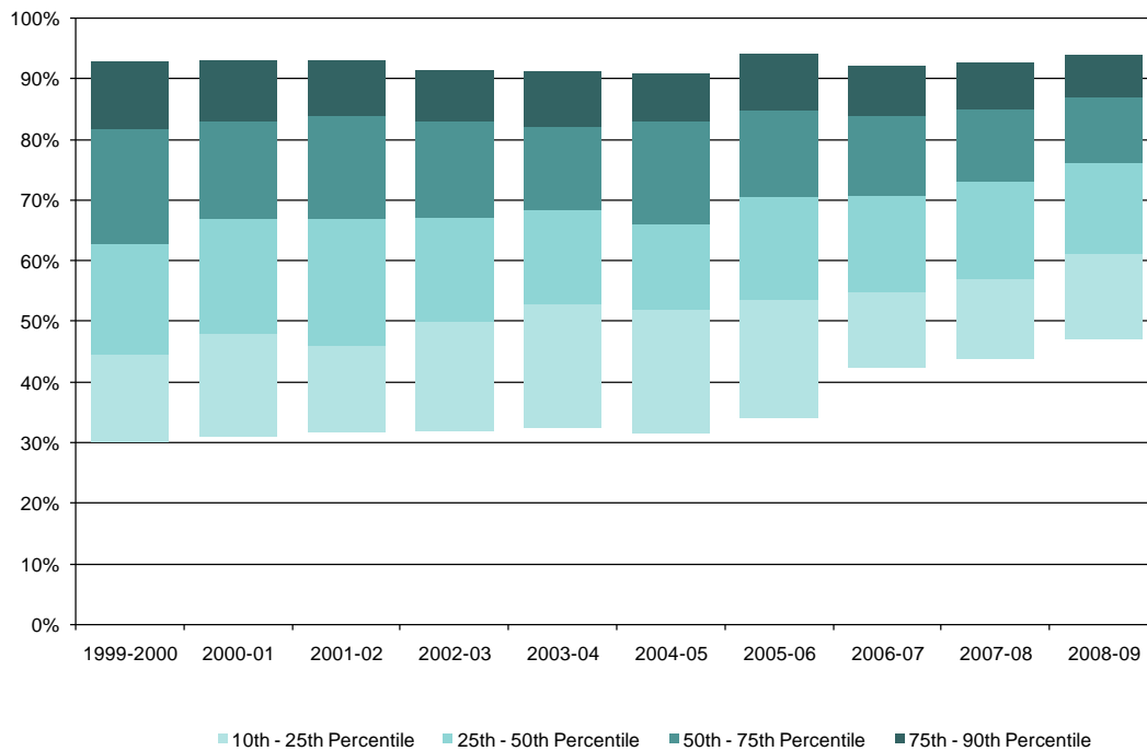
Figure 12: Building condition % GIA condition A and B (C13)
