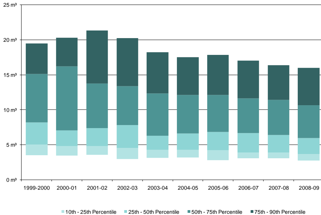
Figure 16: Water consumption (m 3 ) per student and staff FTE (non-residential)
