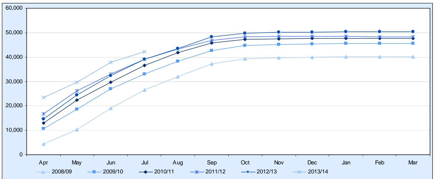
Chart 2: Cumulative number of all TFL applications received, by month and year of study
