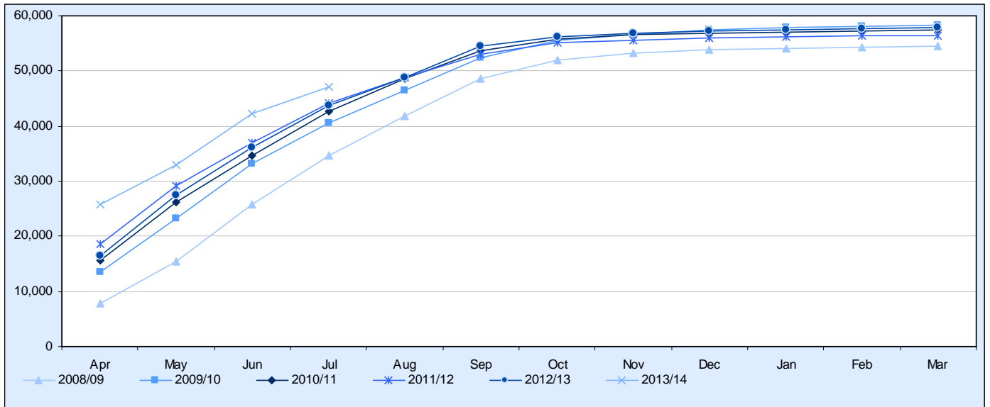
Chart 1: Cumulative number of all student support applications received, by month and year of study
