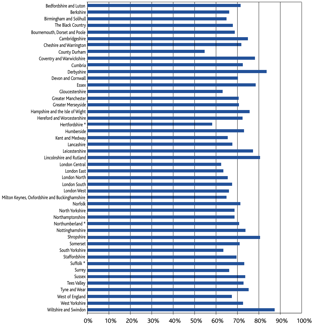
Figure 20. SS 4: Achievement rate: medium qualifications 1999/00 Weighted average of sector colleges by local LSC
