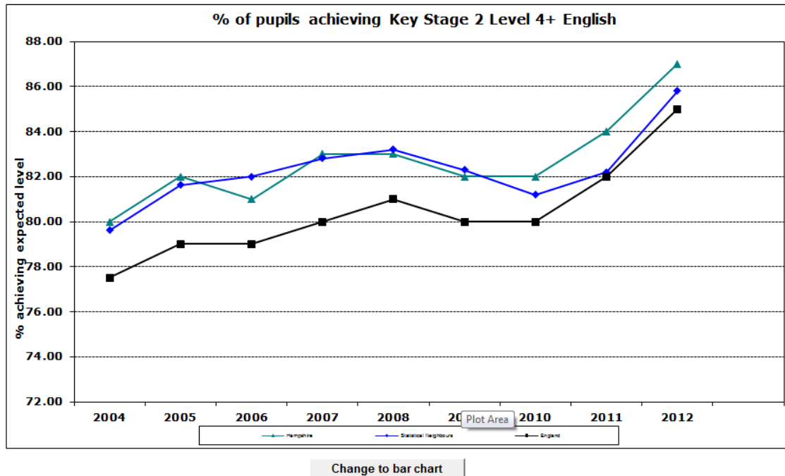
Figure 14: Statistical Neighbour Charting
