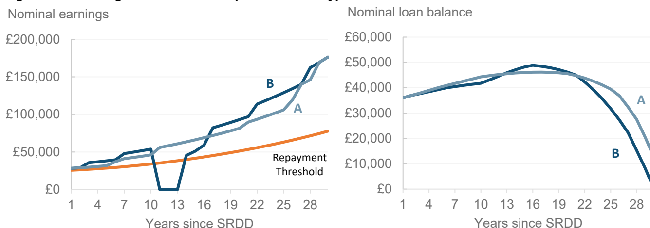
Figure 4.3: Earning and loan balance paths for two hypothetical loan borrowers A and B
