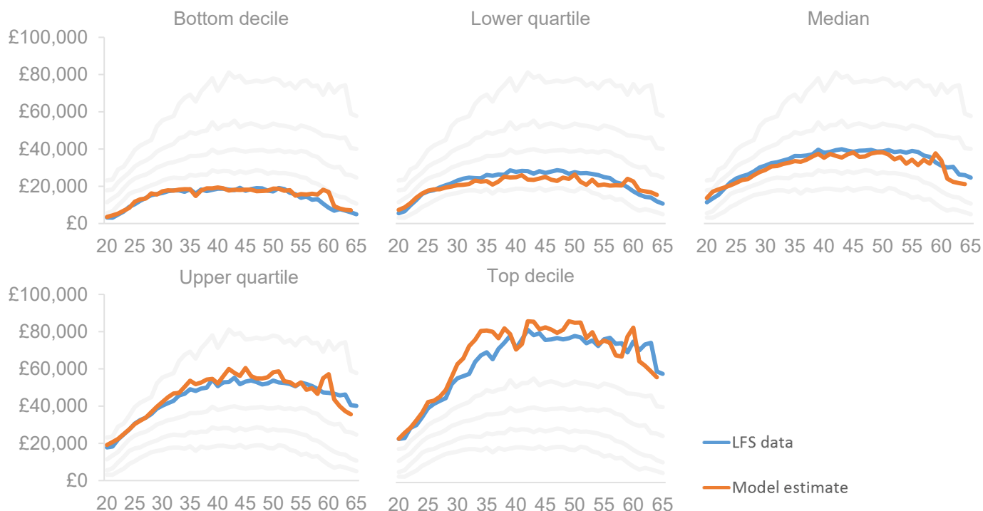
Figure 4.8: The distribution of earnings of male Plan 2 borrowers by age over the working lifetime, estimates compared to distribution observed in LFS data.
